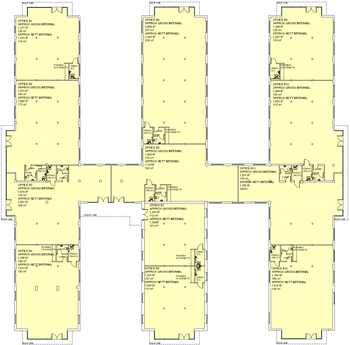
UNIT B FLOOR PLANS
