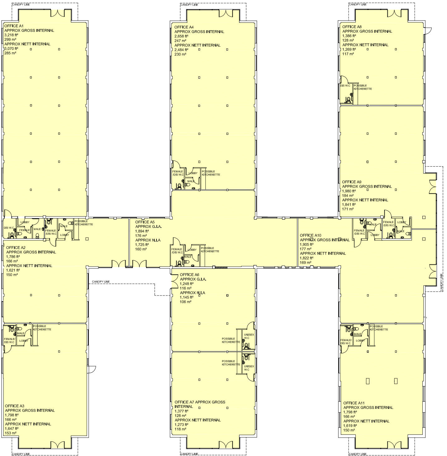
UNIT A FLOOR PLANS
